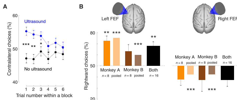
Fig. 3. The effects are stronger for initial stimuli during successive stimulation. (A) Mean \pm SEM choices of the contralateral target as a function of trial number within a block, separately for nonstimulated (black) and stimulated (blue) blocks of trials. Data were pooled across left and right FEF stimulation sites. The asterisks indicate effect significance (two-sided two-sample proportion test; * P < 0.05 , ** P < 0.01 , *** P < 0.001 ). (B) Same format as in Fig. 2B using data of the first three trials of each stimulation block.
