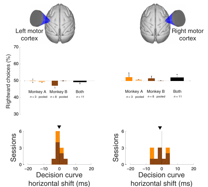
Fig. 5. Stimulation of motor cortex had no effect on choice behavior. Same format as in Figs. 2 and 4, for ultrasound stimulation of left motor cortex (left) and right motor cortex (right).
