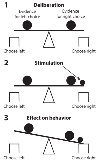
Fig. 6. Decision tasks are sensitive to neuromodulation. Decision-making renders a subject's decision system in a delicate balance between two alternatives. A relatively small perturbation (small filled circle) of the neuronal circuitry representing an alternative has a strong leverage on the subject's decision for that alternative.
