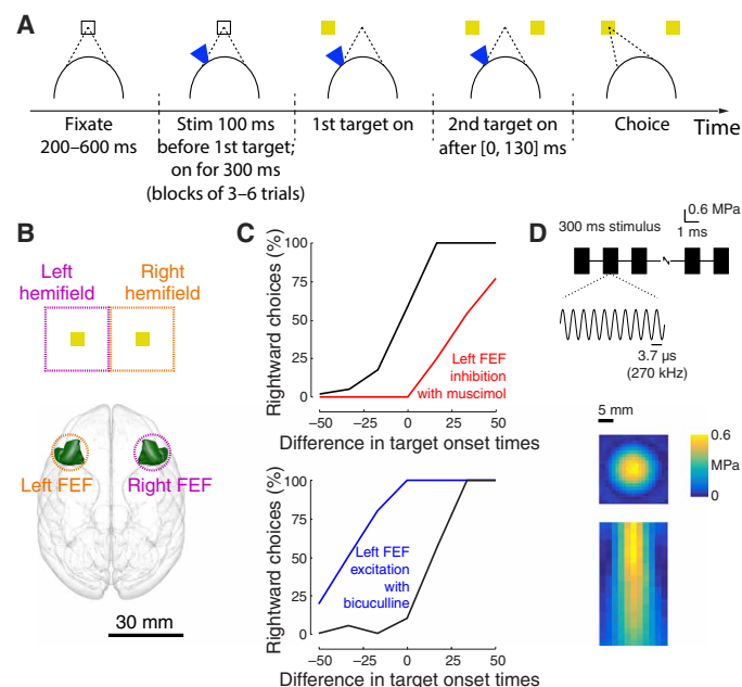
Fig. 1. Choice task and stimulus. (A) Task. The subject fixates a central target. One target appears in the left or the right visual hemifield. After a brief random delay, a second target appears in the opposite hemifield. The subject receives a reward for looking at either target (monkey A) or at the first target (monkey B). Ultrasound is applied in blocks of three to six trials, strictly interleaved with no stimulation blocks of the same duration, 100 ms before the appearance of the first target. (B) Functional characterization of the visuomotor system. We delivered the ultrasound noninvasively (intact skull and skin) into the frontal eye fields (FEF). From anatomical and functional studies, it is known that left/right FEF preferentially represents targets in the right/left visual hemifield. The outline of the FEF was rendered using the Calabrese et al. (50) atlas with Paxinos brain regions. (C) Effects in previous pharmacological neuromodulation studies. When a large amount of strong inhibitory/disinhibitory drugs is injected into the left FEF in this task, animals show a strong ipsilateral/contralateral bias in this task [reproduced from (30), with permission]. These results are as expected given the contralateral nature of the visual hemifield representation and are analogous when other nodes of the visuomotor network, such as the parietal area LIP, are perturbed. (D) Stimulus. The ultrasound stimulus (0.6 MPa, 270 kHz, 300 ms duration) was pulsed at 500 Hz with 1-ms tone burst duration. The ultrasound was applied through a coupling cone filled with agar gel. The resulting pressure, measured in free field, is provided along the lateral (1-mm steps) and axial (2-mm steps) dimensions in color.
