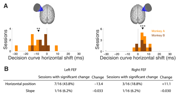
Fig. 4. Biasing nature of the effects. (A) The amount of horizontal shift of the decision curves by ultrasound (blue versus black in Fig. 2A). The data are presented separately for left and right FEF stimulation sessions (left and right panels) and separately for each session in each animal (effect histogram). The orange (brown) counts correspond to sessions of monkey A (B) and the counts are cumulative (no overlap of the orange and brown histograms). The asterisks indicate the effect significance (two-sided t test, **P < 0.01 , ***P < 0.001 ). (B) The table shows the number of sessions (left columns) in which the parameters fitted to each decision curve (rows) changed significantly during ultrasound stimulation. See Materials and Methods for details of the statistical test. The right column shows the average magnitude of the change over the significant sessions. Horizontal position is measured in milliseconds and slope is measured in per millisecond.
