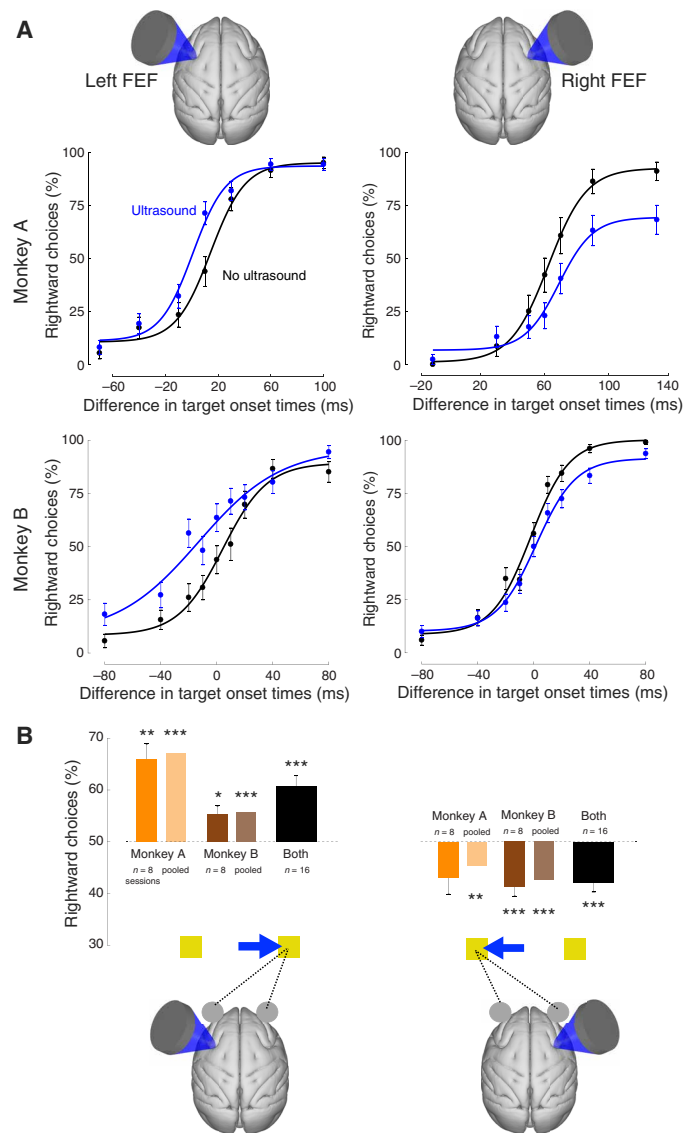
Fig. 2. Effects of ultrasonic stimulation on choice behavior. (A) Single-session examples. Mean ( \pm SEM) proportion of choices of the rightward target as a function of the difference in target onset times. Positive difference stands for the cases in which the rightward target appeared first. The black data points reflect choice behavior in the trials in which the animal was not stimulated, whereas the blue data points represent choice behavior in the stimulated trials. The data were fit with a four-parameter sigmoid function (see Materials and Methods). The data are presented separately for left and right FEF stimulation sessions (left and right columns; see illustration on top) and for monkeys A and B (top and bottom rows). (B) Quantification of the effects for all sessions. No stimulation data were fit with the sigmoid function [black curves in (A)]. Using the fit, we identified the time difference on the abscissa for which the animal chose both targets in equal proportion (see Materials and Methods). At that point, we then assessed the proportion of rightward choices during the stimulated trials. This analysis was performed for each individual session (dark bars) and for data pooled over the sessions (light bars). The number of sessions is provided in the inset. Asterisks indicate the cases in which the mean effects statistically differ from equal preference [two-sided t test for individual sessions (dark bars) and randomization test for data pooled across sessions (light bars)]. * P < 0.05, ** P < 0.01, *** P < 0.001. The illustration on the bottom summarizes the polarity of the biasing effects.
